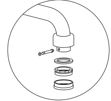
Concealed brass fixing mechanism
