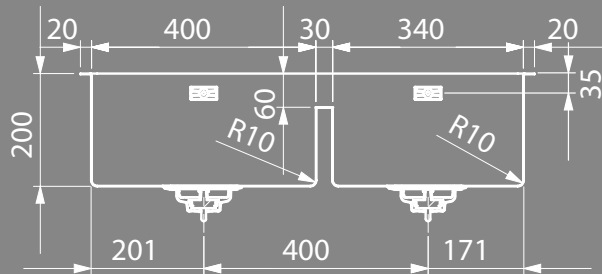
Sopratop Overmount
