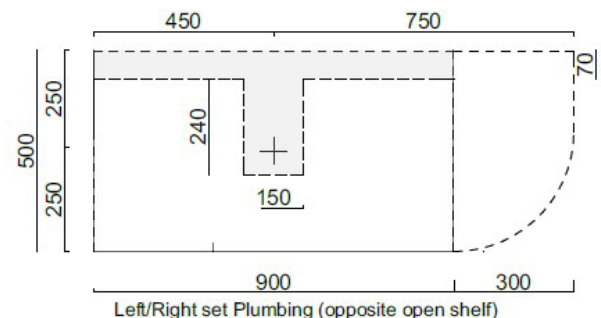
Left/Right set Plumbing (opposite open shelf)
