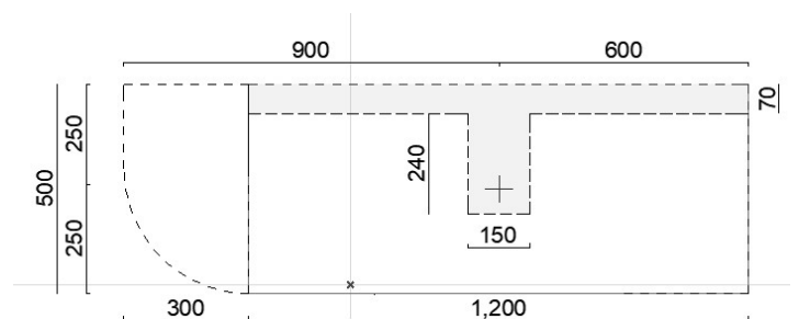
Left /right set plumbing -opposite open shelves
