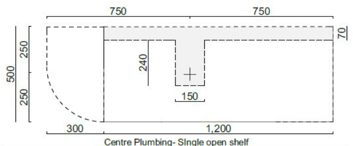
Centre Plumbing- Single open shelf
